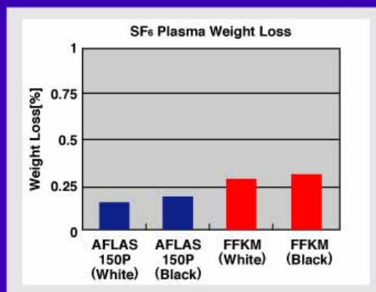
Fig3. Weight loss by SF 6 plasma
