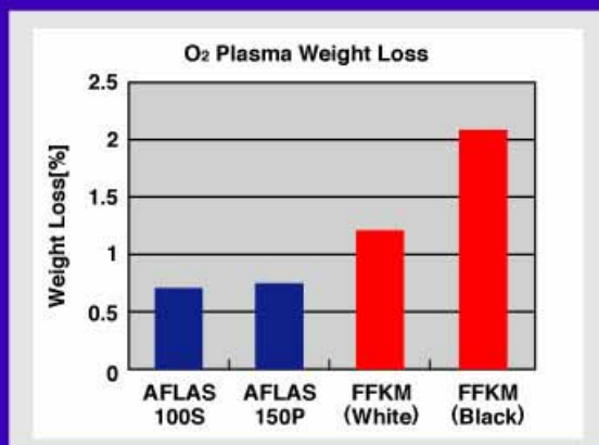
Fig1. Weight loss by O 2 plasma
