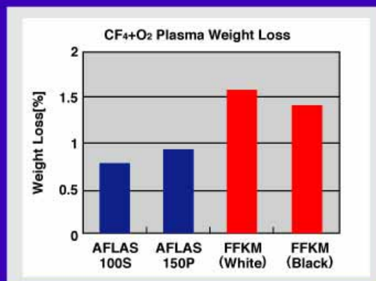
Fig2. Weight loss by CF 4 +O 2 plasma
